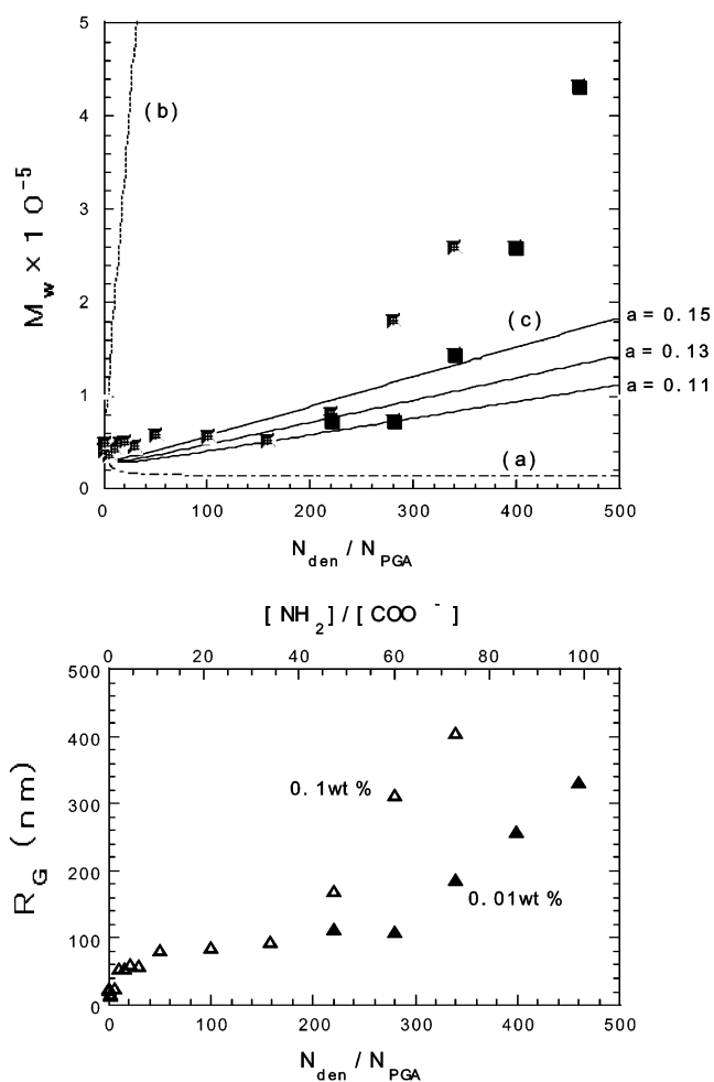
Figure 2. M_w and R_G for mixed solutions of PAMAM dendrimer and NaPGA in 0.25 M NaCl as a function of N_{den}/N_{PGA} . (Top) Observed M_w : ■, 0.01 wt % NaPGA; □, 0.1 wt % NaPGA. Calculated M_w : (a) a nonbinding model; (b) an average binding model; (c) a distribution-binding model at a = 0.11 , 0.13, and 0.15. (Bottom) Observed R_G : ▲, 0.01 wt % NaPGA; △, 0.1 wt % NaPGA.
