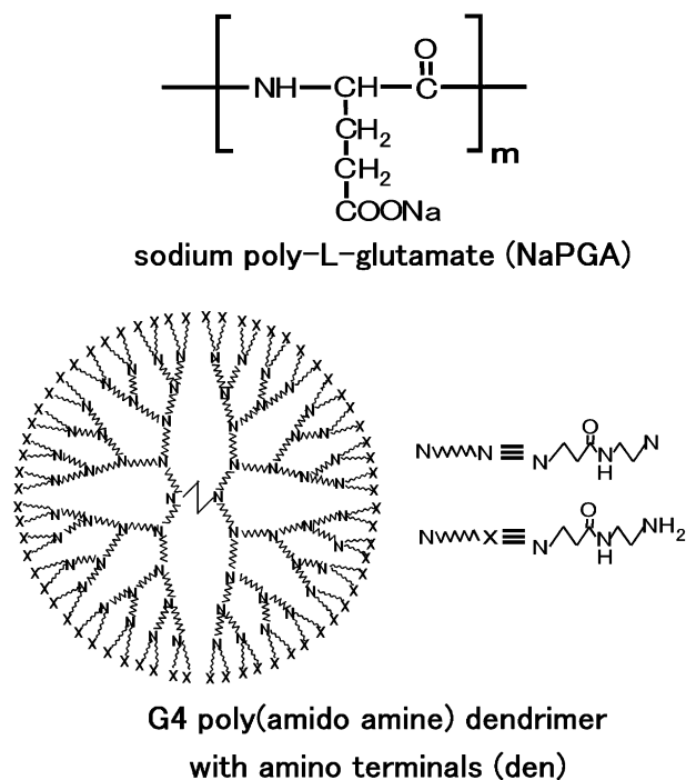
Figure 1. Chemical structures of a repeating unit of sodium poly-L-glutamate (NaPGA) (top) and a fourth-generation amino-terminated poly(amido amine) (G4 PAMAM) dendrimer (bottom).
