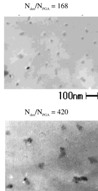
Figure 7. TEM photographs of specimens prepared from mixed solutions of PAMAM dendrimer and NaPGA in 0.25 M NaCl at N_{\text{den}}/N_{\text{PGA}} = 168 and 420.
