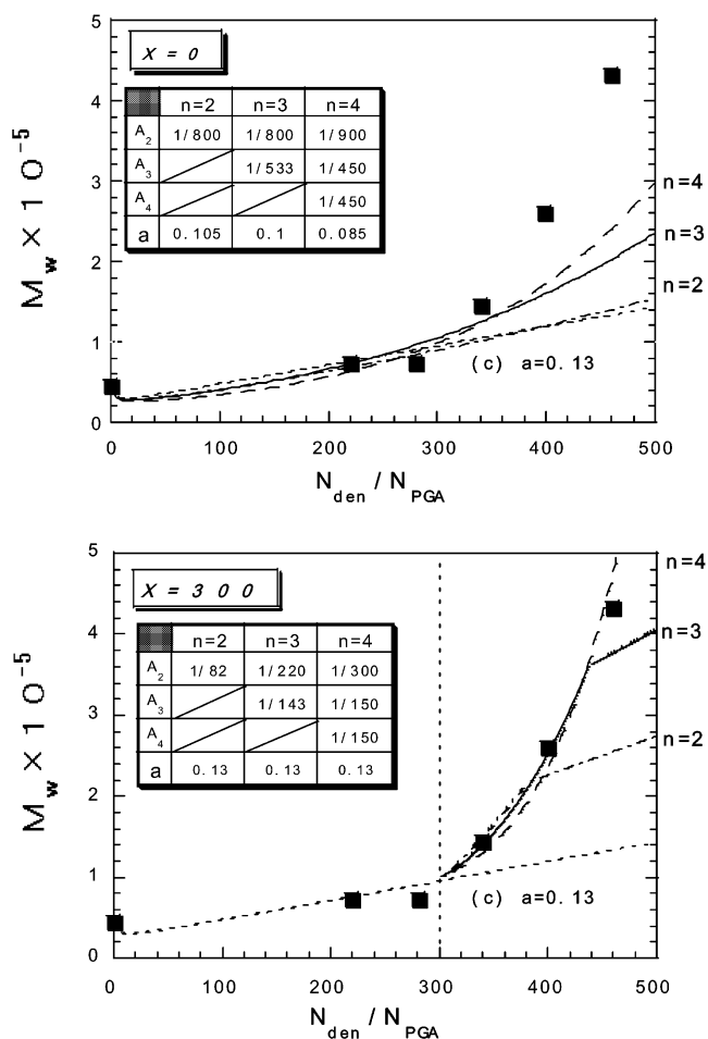
Figure 5. Calculation of M_w for mixed solutions of PAMAM dendrimer and NaPGA in 0.25 M NaCl as a function of N_{\text{den}}/N_{\text{PGA}} on the basis of the aggregation model. NaPGA concentration, 0.01 wt %. ■, observed. The optimum parameters for the best fitting are included in the figures.
